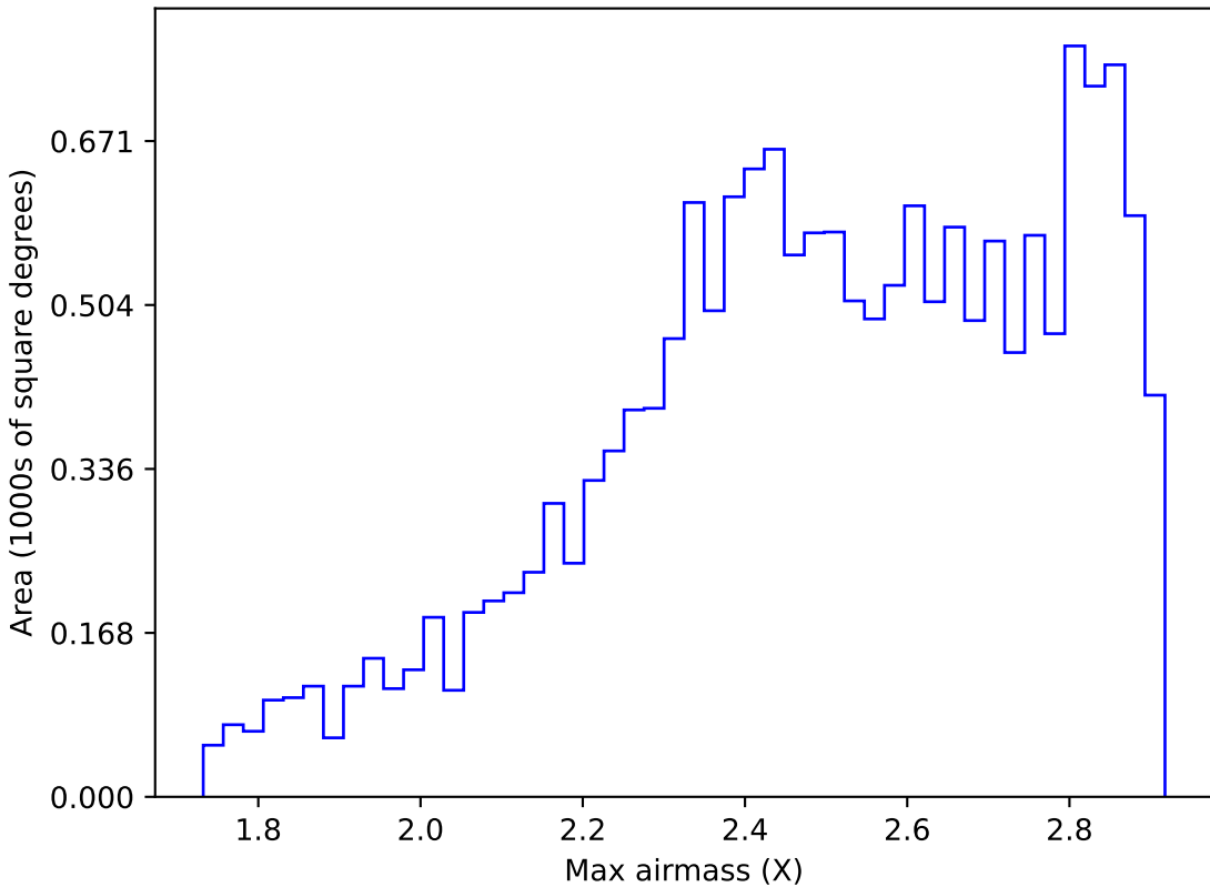
no_magell_roll_v3.4_10yrs WFD z band: Max airmass
