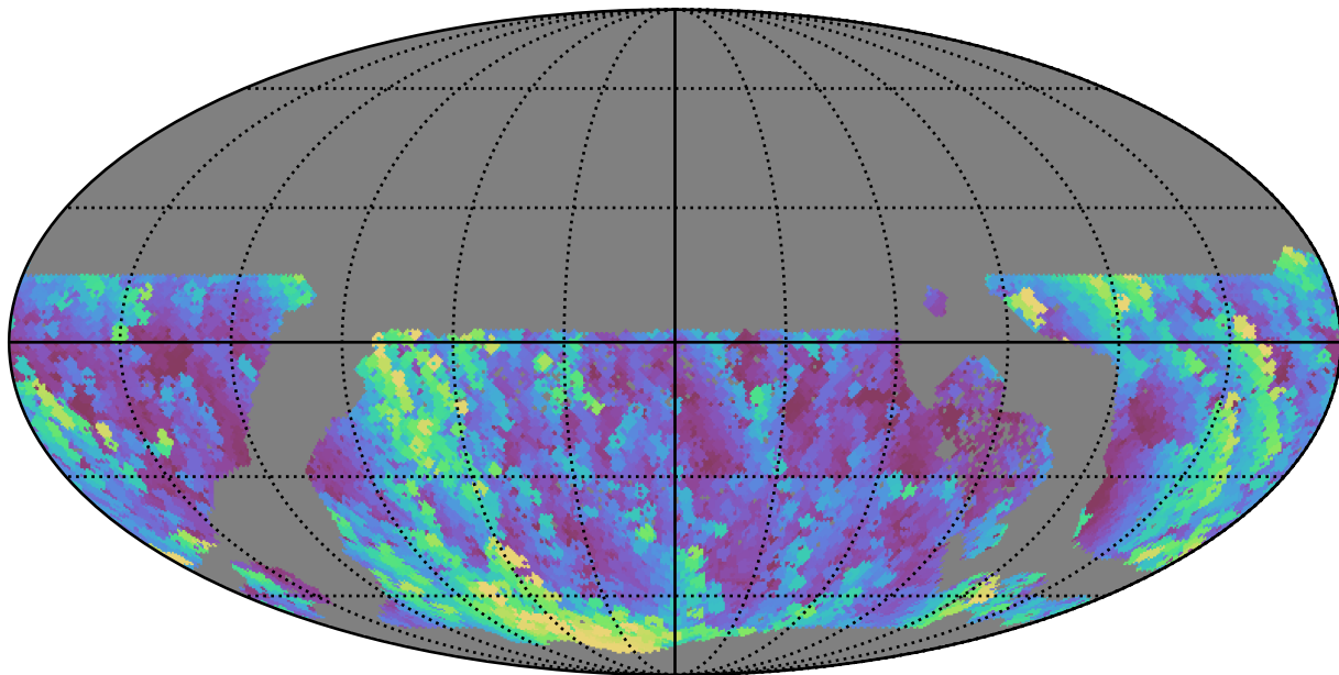
no_magell_roll_v3.4_10yrs WFD u band: Max airmass
