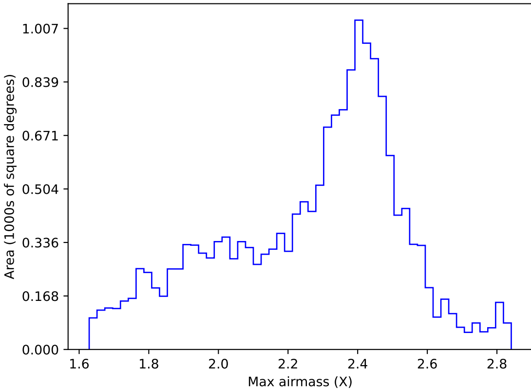
no_magell_roll_v3.4_10yrs WFD r band: Max airmass
