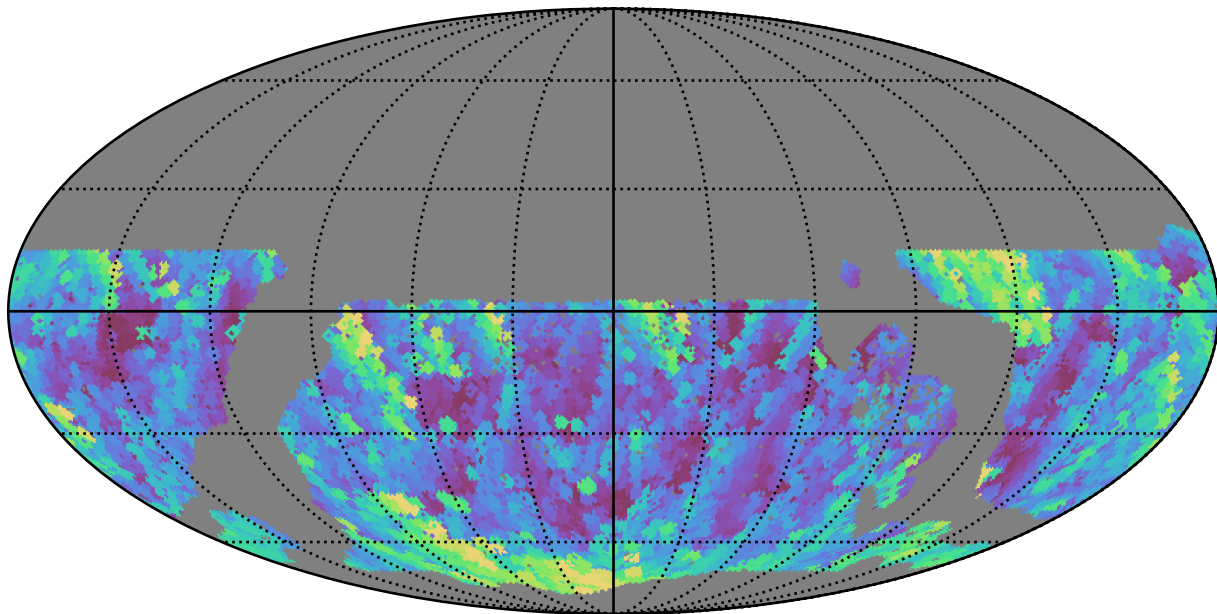
no_magell_roll_v3.4_10yrs WFD g band: Max airmass
