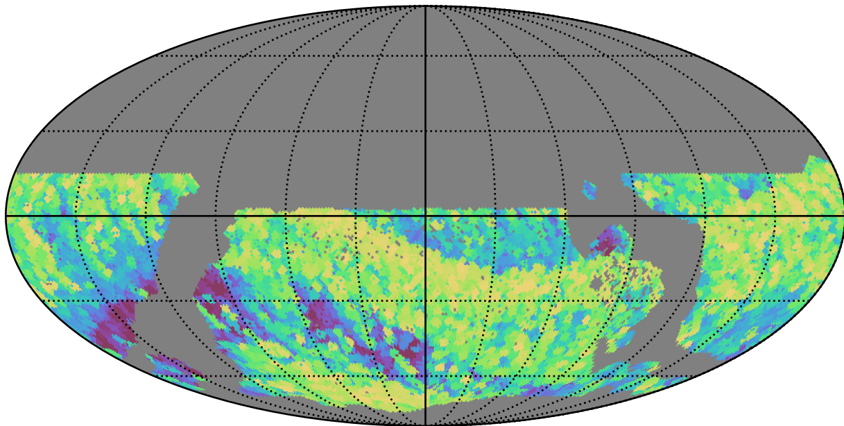
no_magell_roll_v3.4_10yrs WFD all bands: Max airmass
