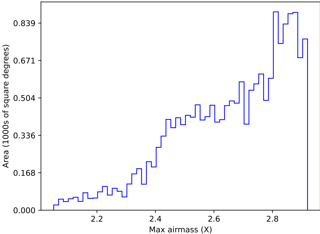
no_magell_roll_v3.4_10yrs WFD all bands: Max airmass
