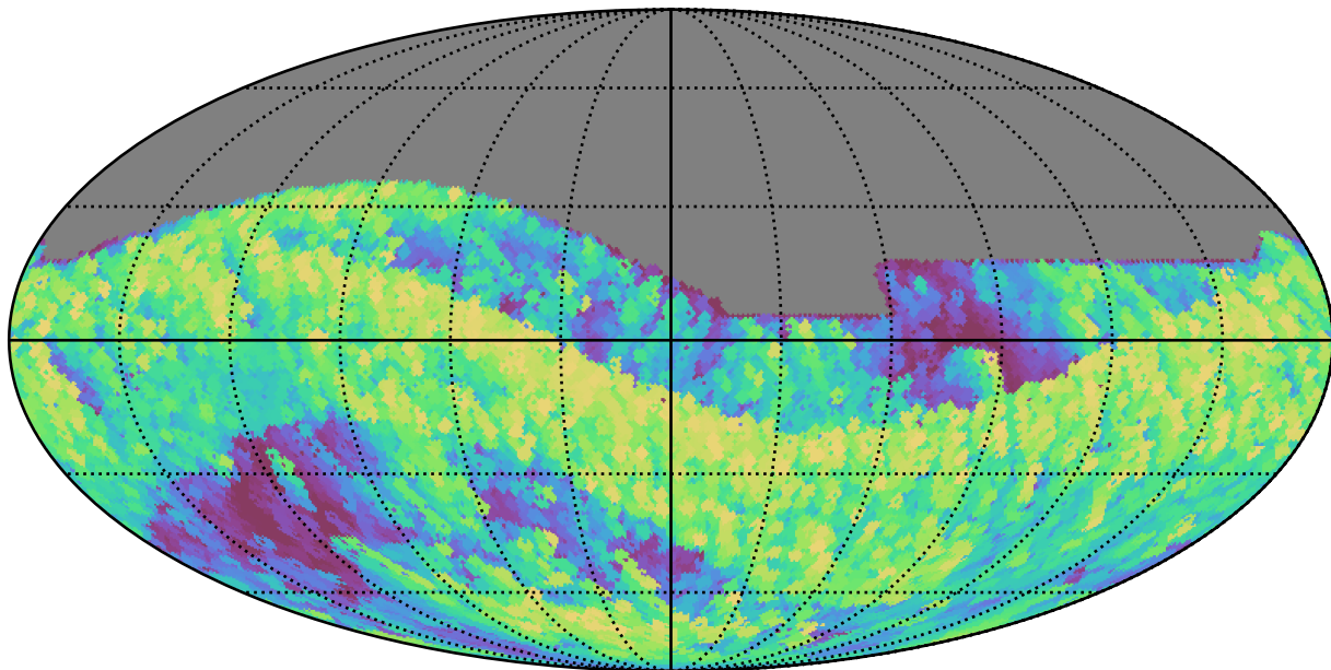
no_magell_roll_v3.4_10yrs All sky z band: Max airmass
