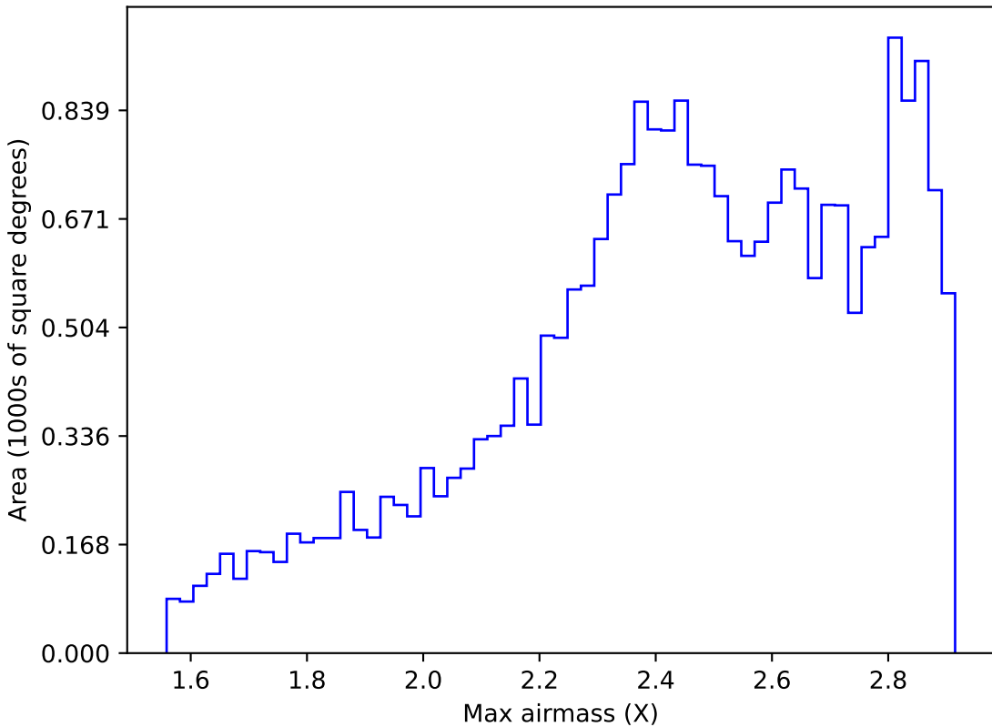
no_magell_roll_v3.4_10yrs All sky z band: Max airmass
