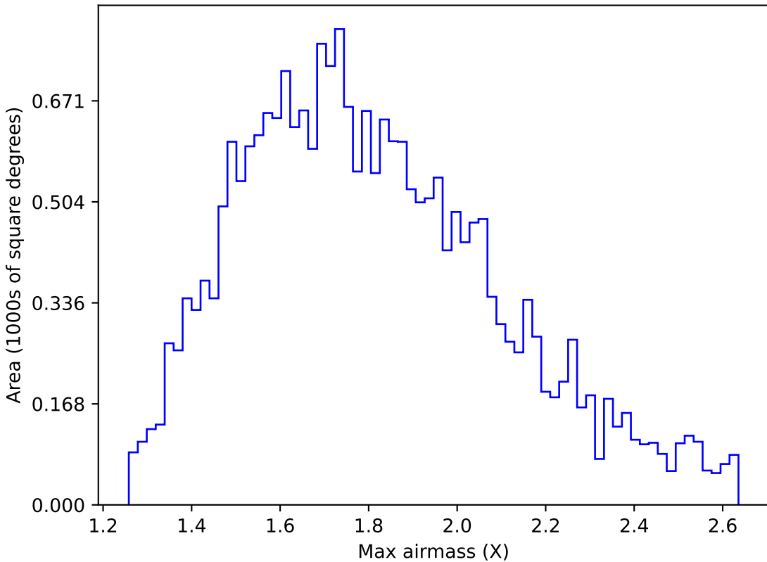
no_magell_roll_v3.4_10yrs All sky u band: Max airmass
