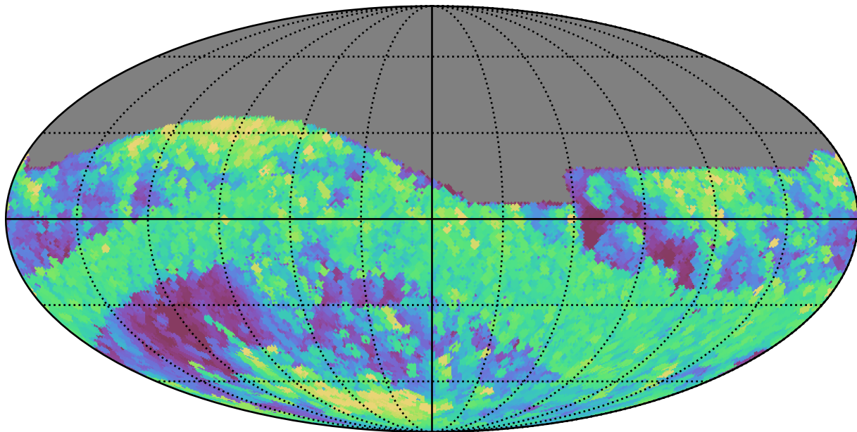
no_magell_roll_v3.4_10yrs All sky r band: Max airmass
