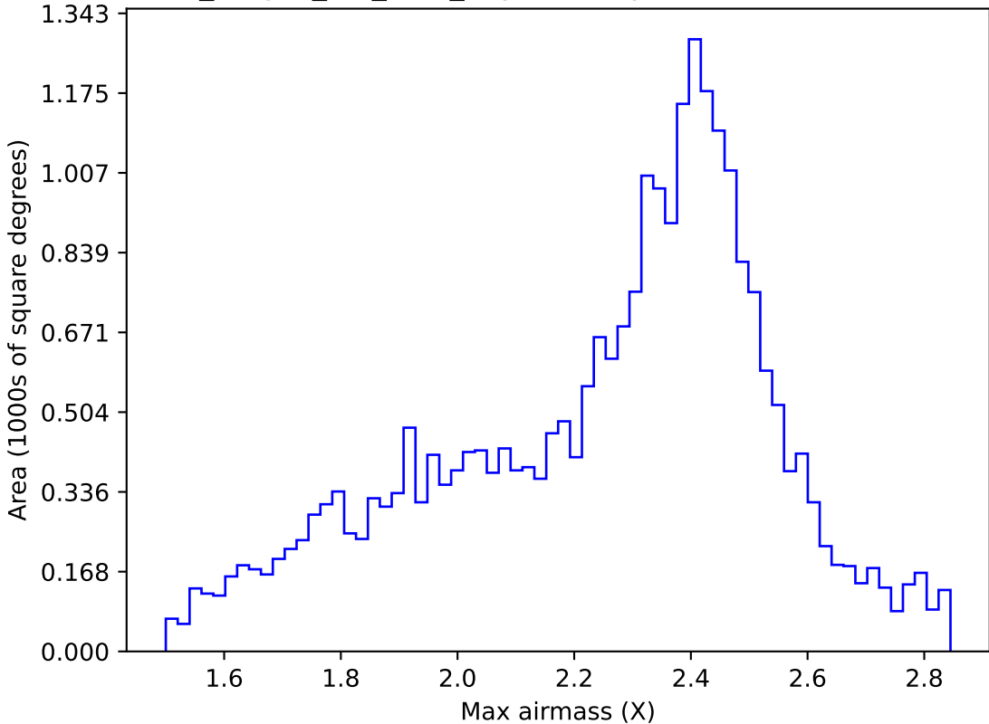
no_magell_roll_v3.4_10yrs All sky r band: Max airmass
