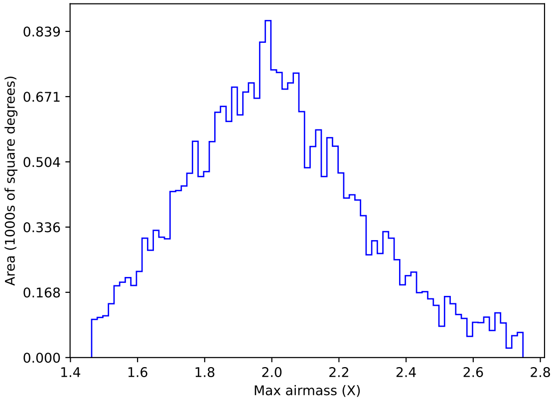
no_magell_roll_v3.4_10yrs All sky g band: Max airmass
