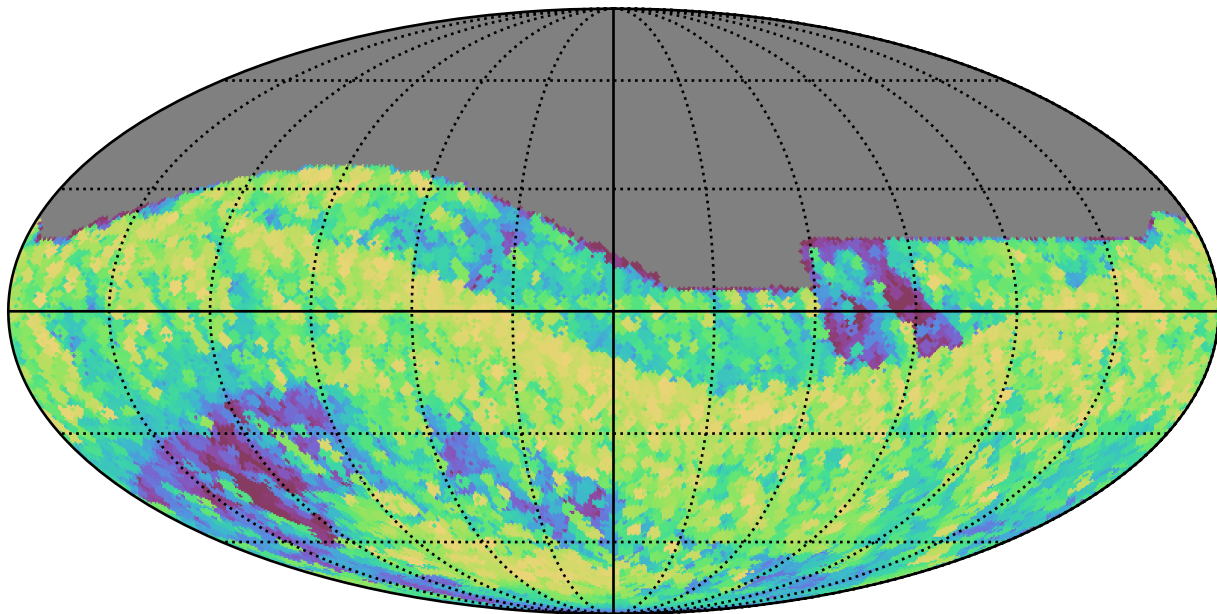
no_magell_roll_v3.4_10yrs All sky all bands: Max airmass
