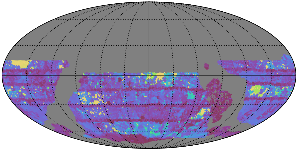
no_magell_roll_v3.4_10yrs WFD z band: Max Inter-Night Gap
