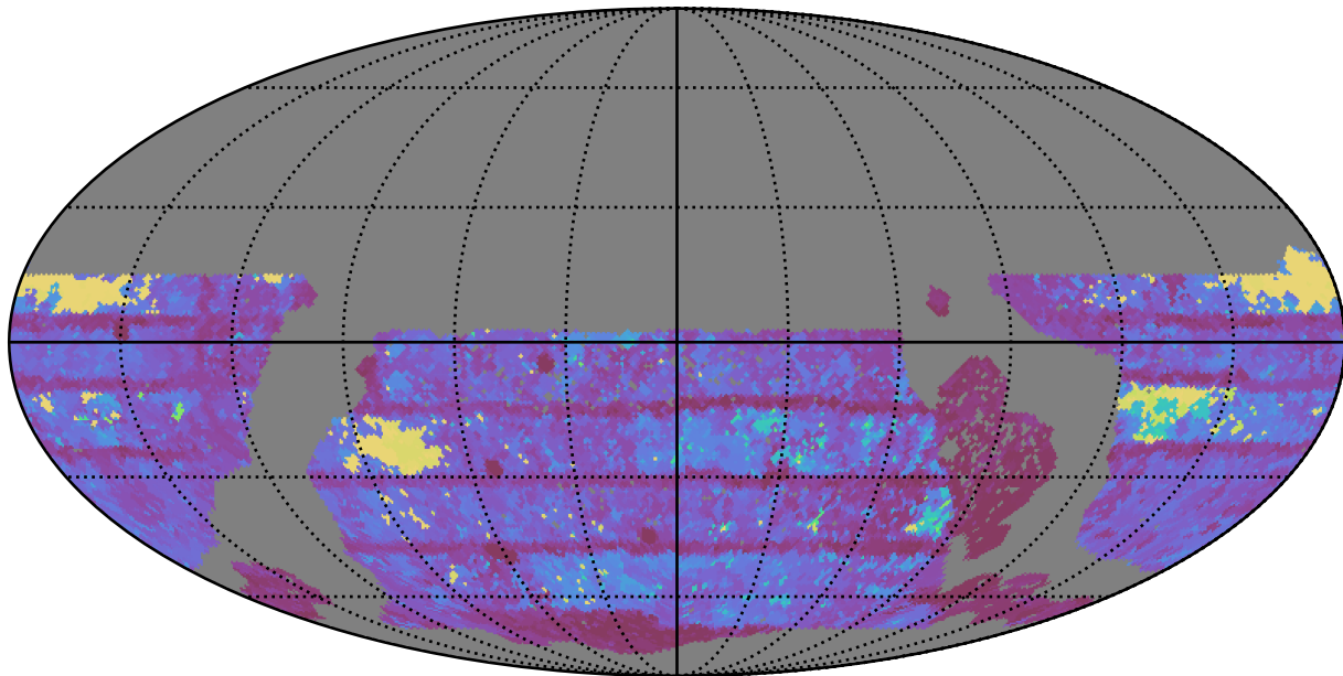
no_magell_roll_v3.4_10yrs WFD r band: Max Inter-Night Gap
