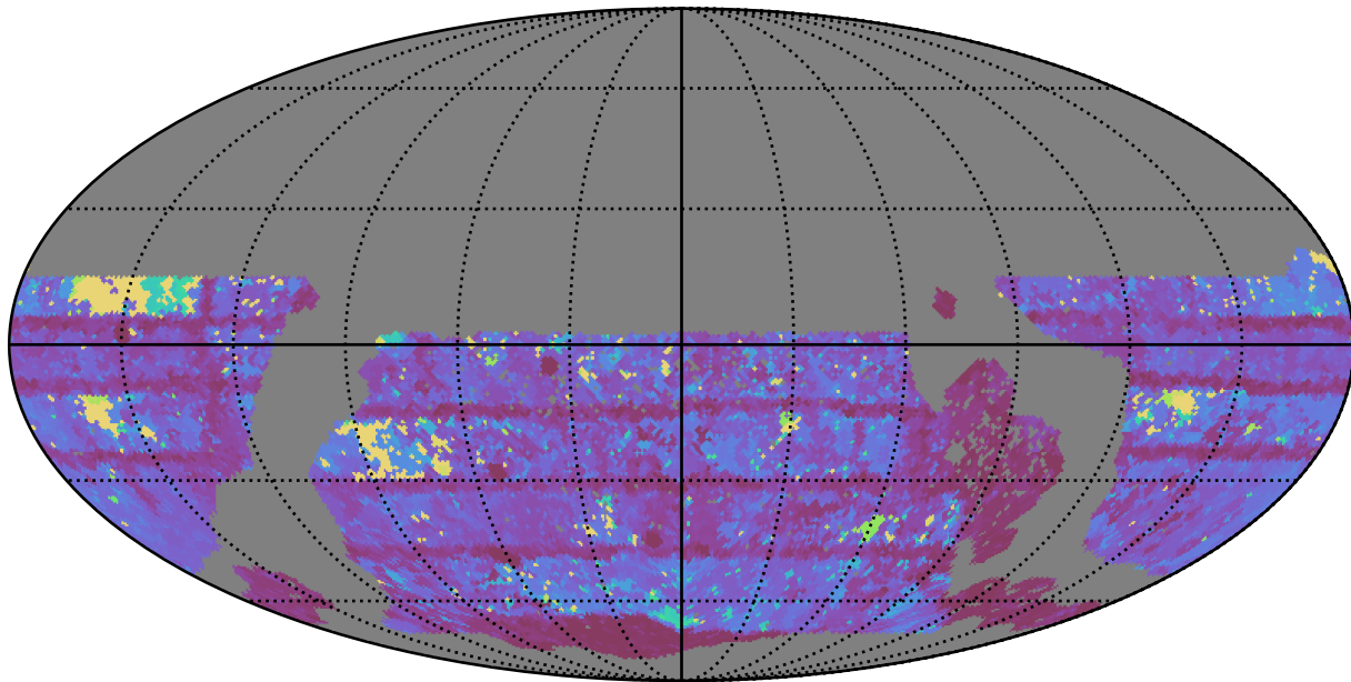
no_magell_roll_v3.4_10yrs WFD i band: Max Inter-Night Gap
