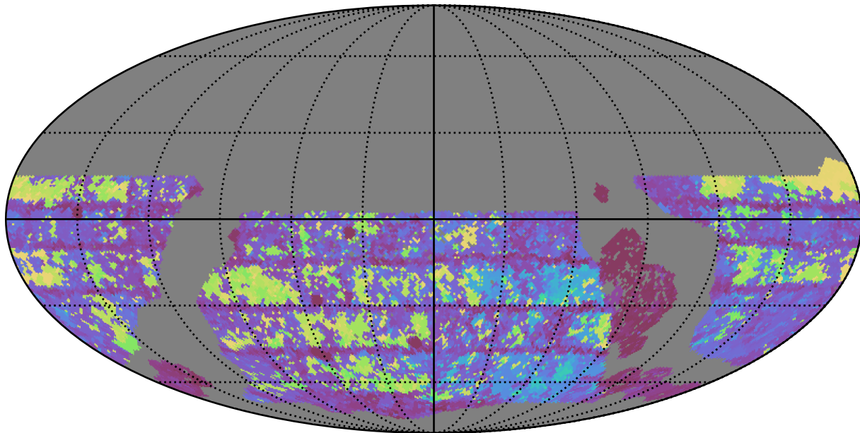
no_magell_roll_v3.4_10yrs WFD g band: Max Inter-Night Gap
