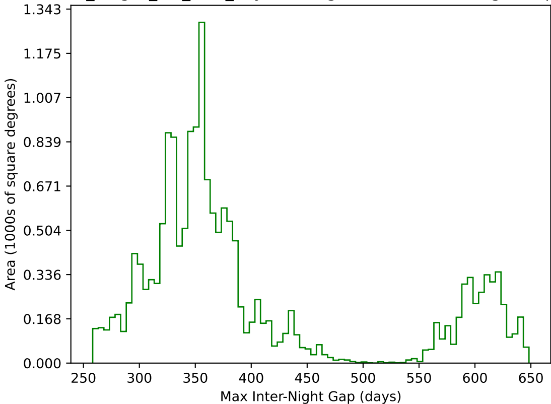
no_magell_roll_v3.4_10yrs WFD g band: Max Inter-Night Gap
