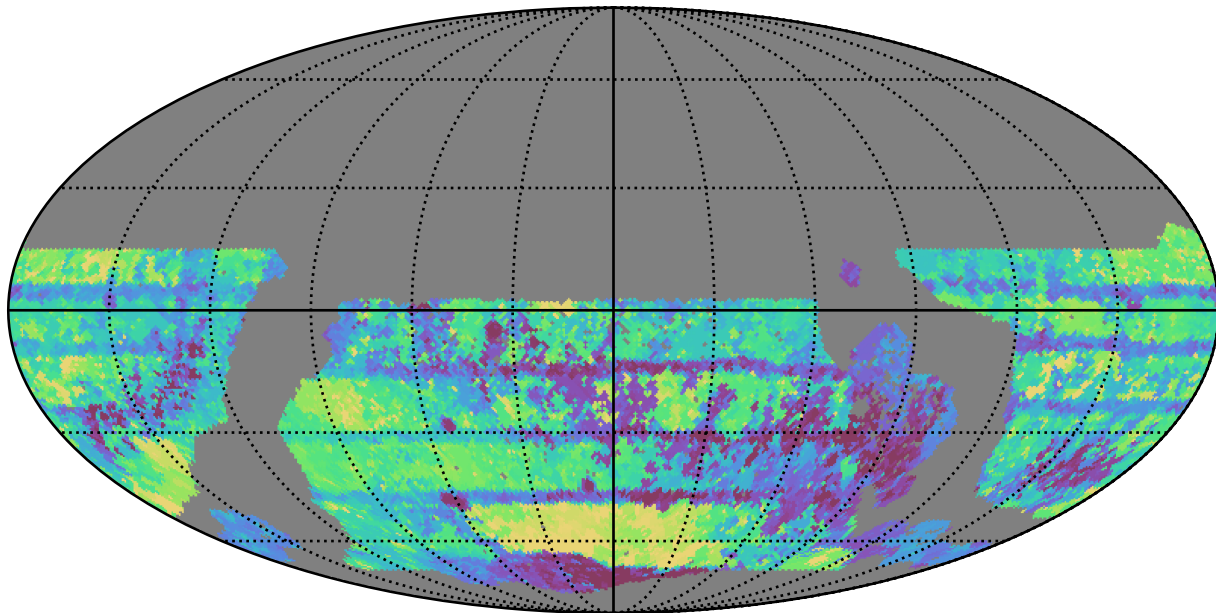
no_magell_roll_v3.4_10yrs WFD all bands: Max Inter-Night Gap
