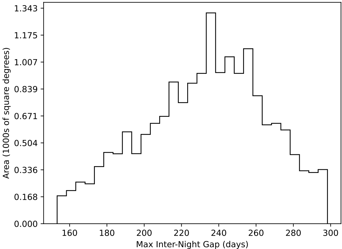
no_magell_roll_v3.4_10yrs WFD all bands: Max Inter-Night Gap
