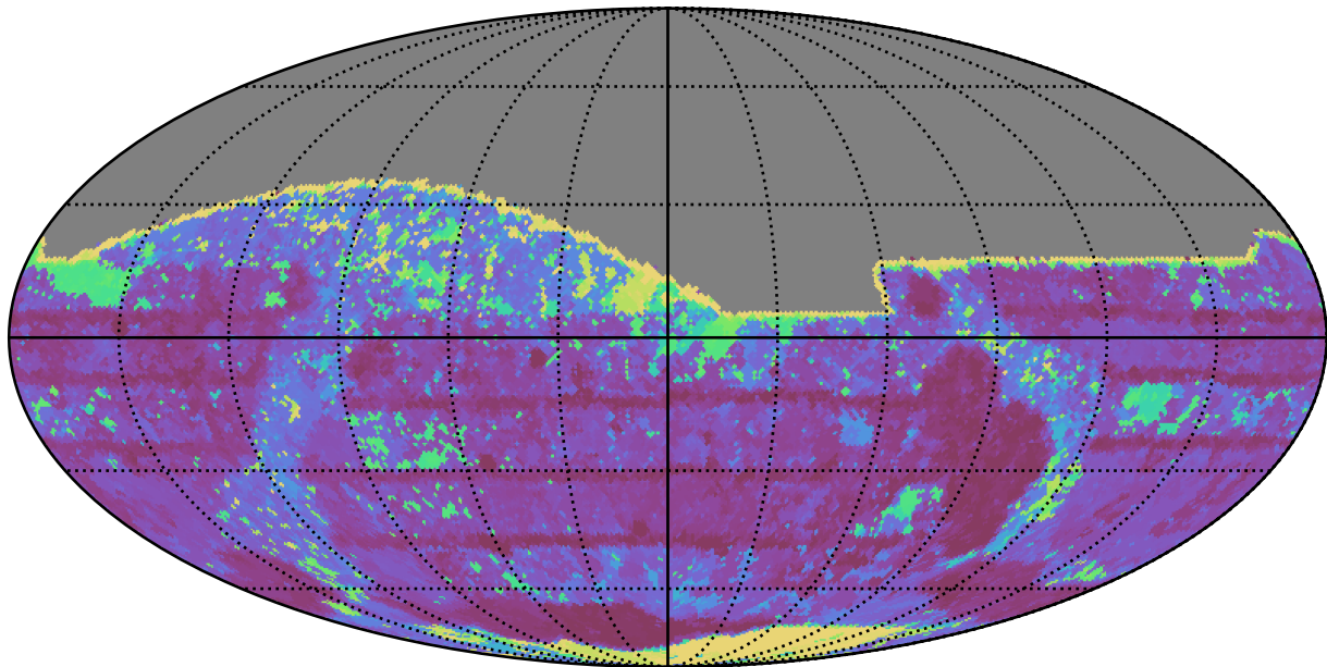
no_magell_roll_v3.4_10yrs All sky z band: Max Inter-Night Gap
