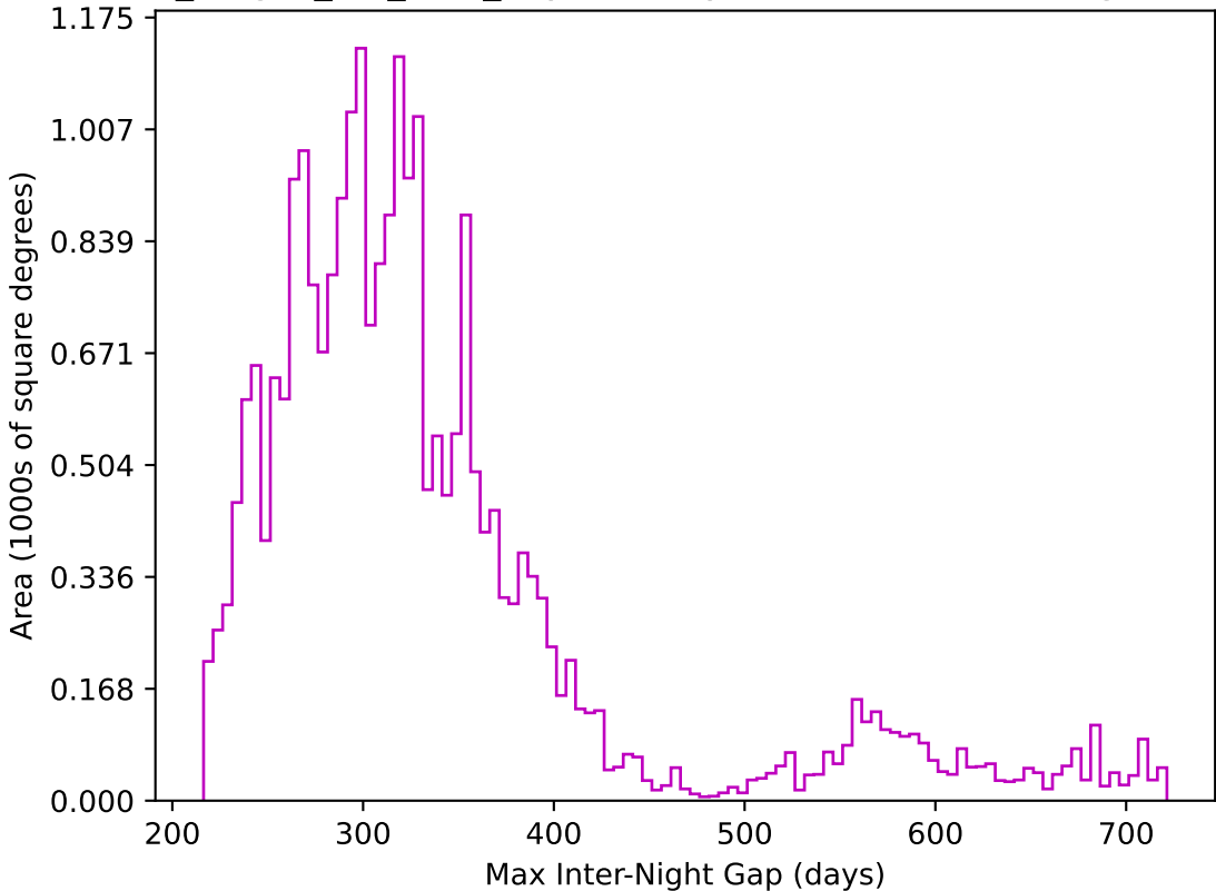
no_magell_roll_v3.4_10yrs All sky z band: Max Inter-Night Gap
