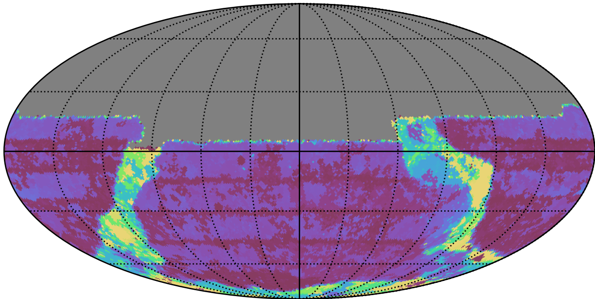
no_magell_roll_v3.4_10yrs All sky u band: Max Inter-Night Gap
