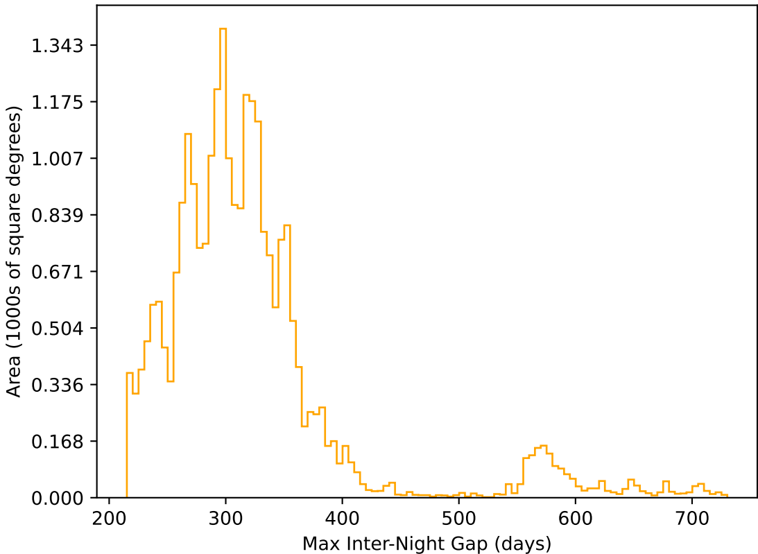
no_magell_roll_v3.4_10yrs All sky r band: Max Inter-Night Gap
