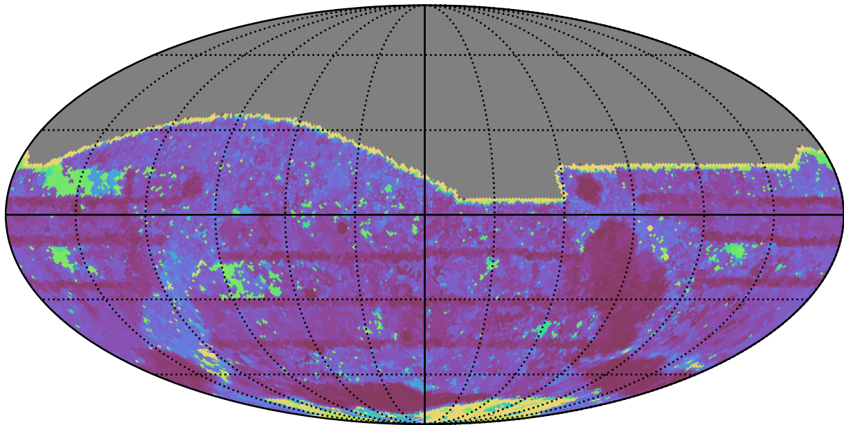
no_magell_roll_v3.4_10yrs All sky i band: Max Inter-Night Gap
