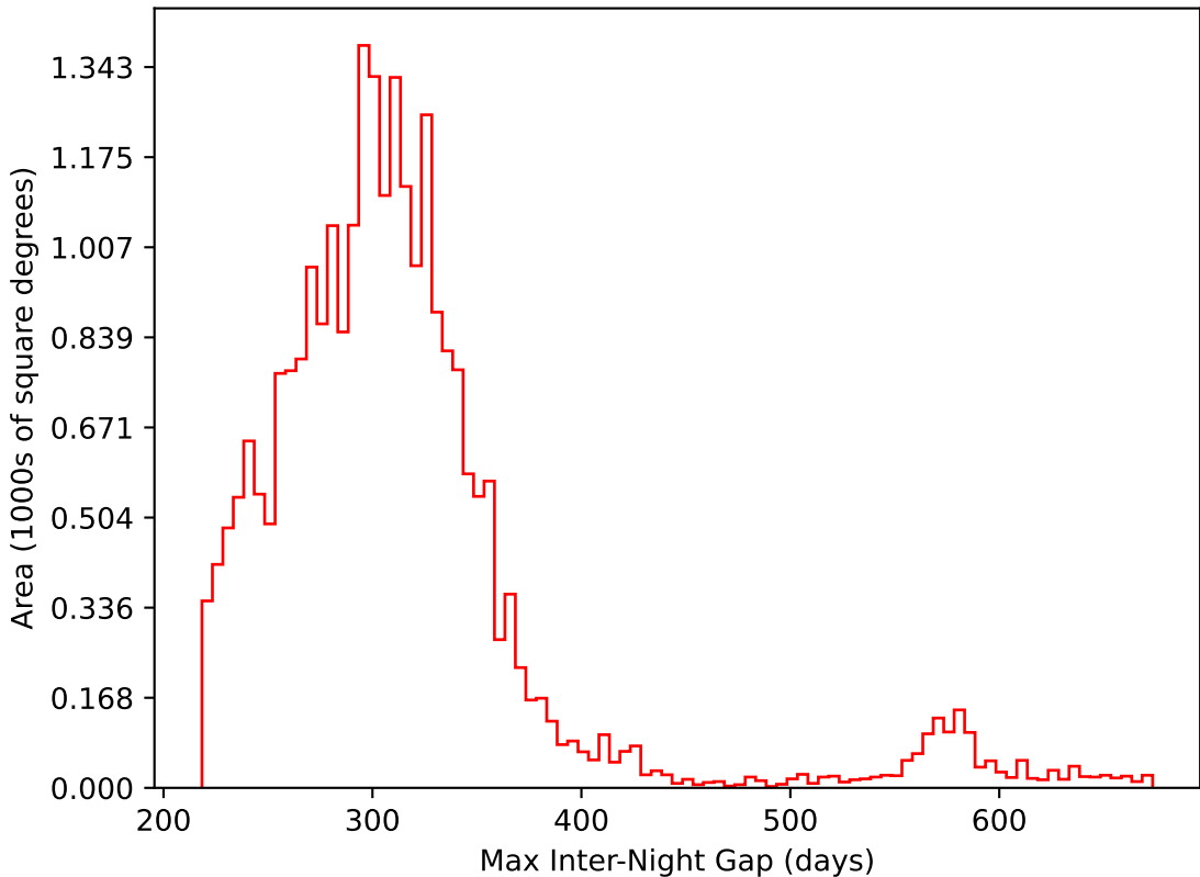
no_magell_roll_v3.4_10yrs All sky i band: Max Inter-Night Gap
