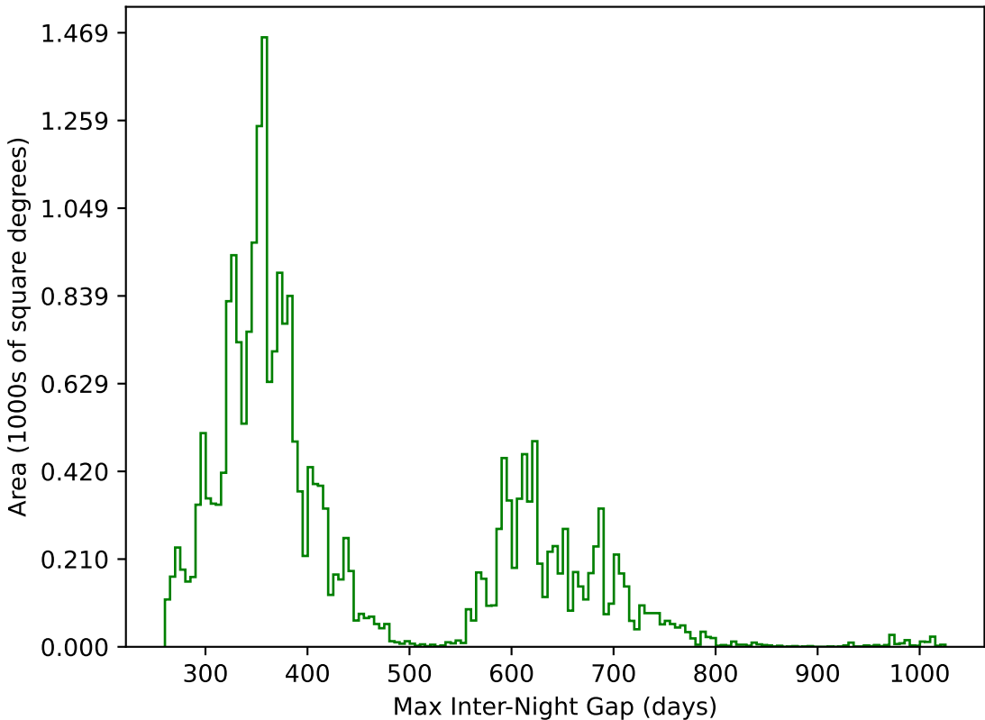
no_magell_roll_v3.4_10yrs All sky g band: Max Inter-Night Gap
