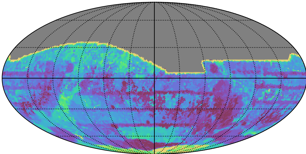
no_magell_roll_v3.4_10yrs All sky all bands: Max Inter-Night Gap
