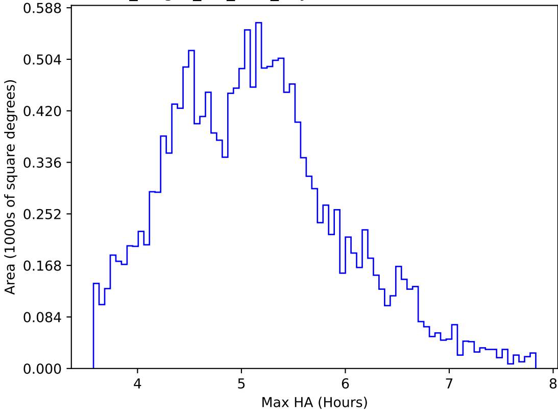
no_magell_roll_v3.4_10yrs WFD all bands: Max HA
