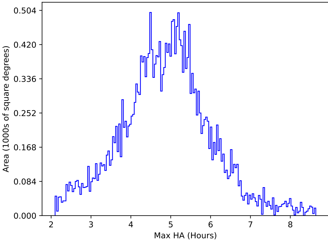
no_magell_roll_v3.4_10yrs All sky all bands: Max HA
