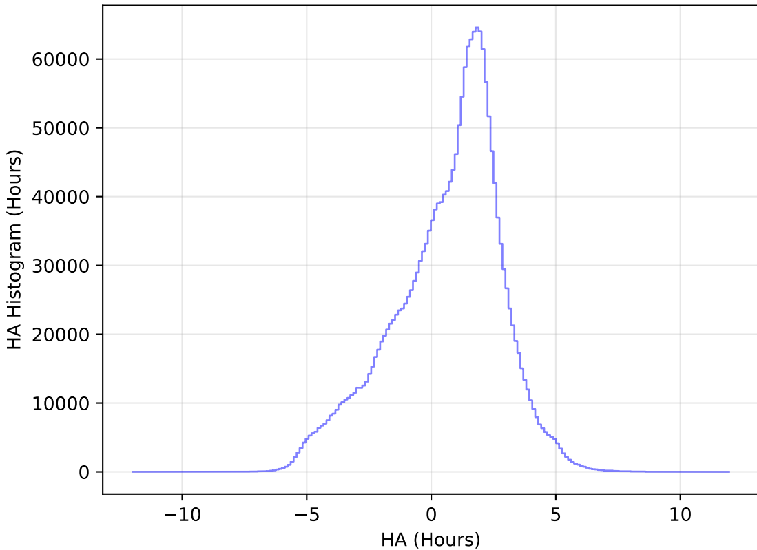
no_magell_roll_v3.4_10yrs All sky all bands: HA Histogram
