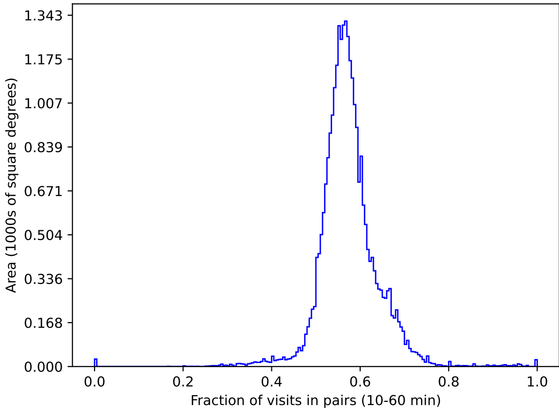
no_magell_roll_v3.4_10yrs gri All sky: Fraction of visits in pairs (10-60 min)
