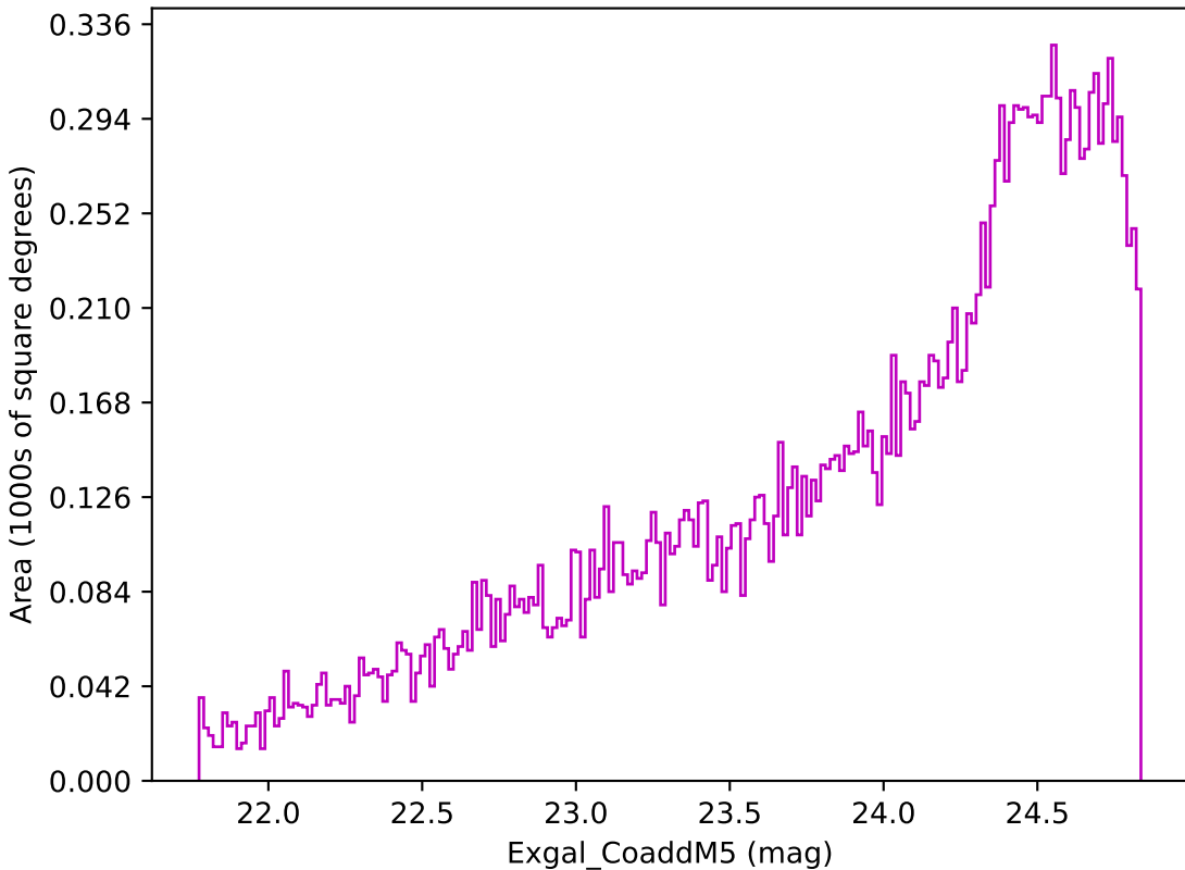
no_magell_roll_v3.4_10yrs Yr 3-4 z band: Exgal_CoaddM5
