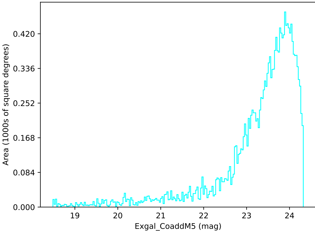
no_magell_roll_v3.4_10yrs Yr 3-4 u band: Exgal_CoaddM5
