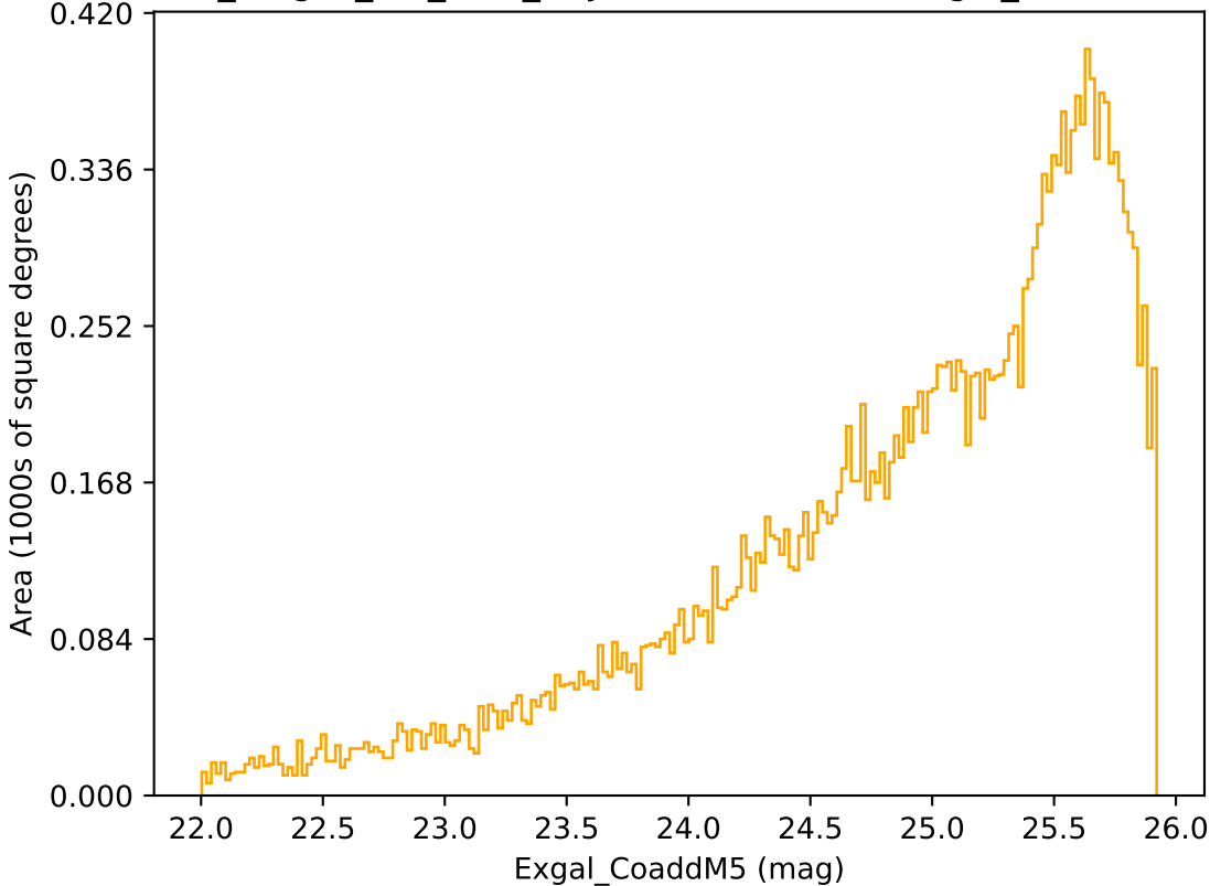
no_magell_roll_v3.4_10yrs Yr 3-4 r band: Exgal_CoaddM5
