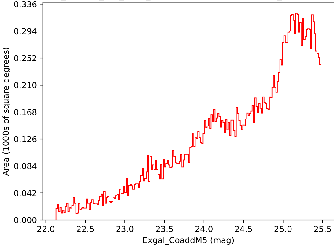
no_magell_roll_v3.4_10yrs Yr 3-4 i band: Exgal_CoaddM5
