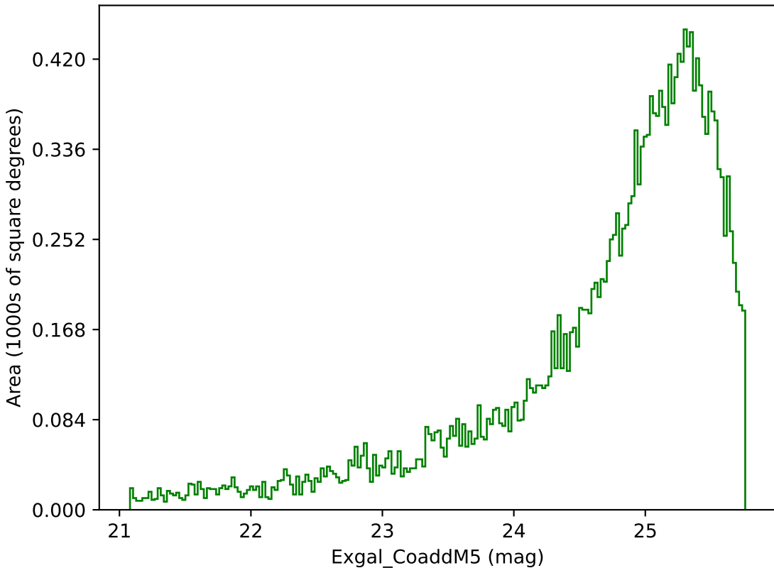
no_magell_roll_v3.4_10yrs Yr 3-4 g band: Exgal_CoaddM5
