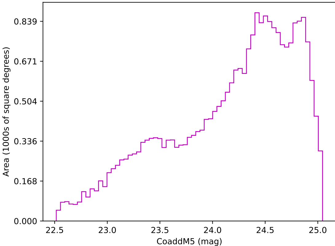
no_magell_roll_v3.4_10yrs Yr 3-4 z band: CoaddM5
