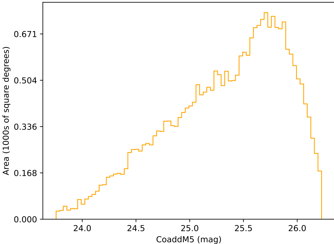
no_magell_roll_v3.4_10yrs Yr 3-4 r band: CoaddM5
