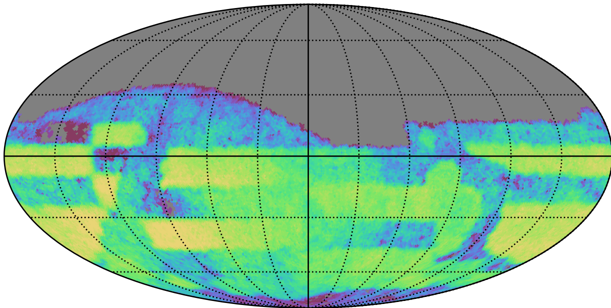
no_magell_roll_v3.4_10yrs Yr 3-4 i band: CoaddM5
