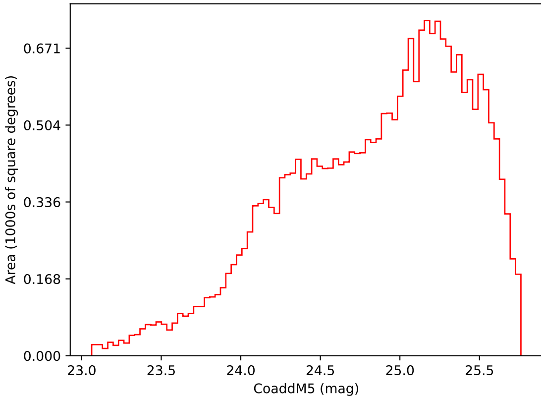
no_magell_roll_v3.4_10yrs Yr 3-4 i band: CoaddM5
