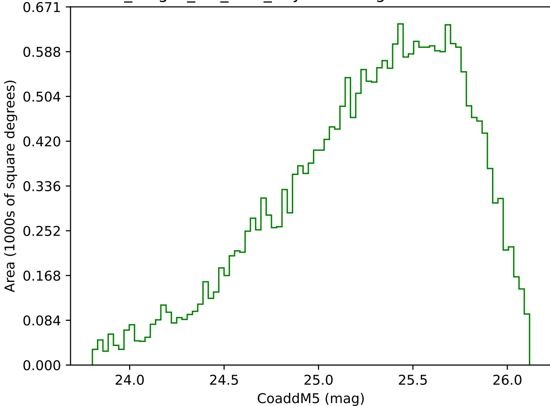
no_magell_roll_v3.4_10yrs Yr 3-4 g band: CoaddM5
