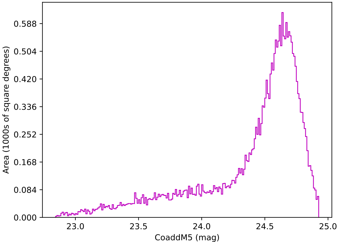
no_magell_roll_v3.4_10yrs Yr 1 z band: CoaddM5
