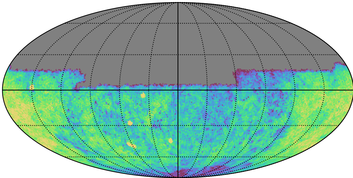
no_magell_roll_v3.4_10yrs Yr 1 u band: CoaddM5
