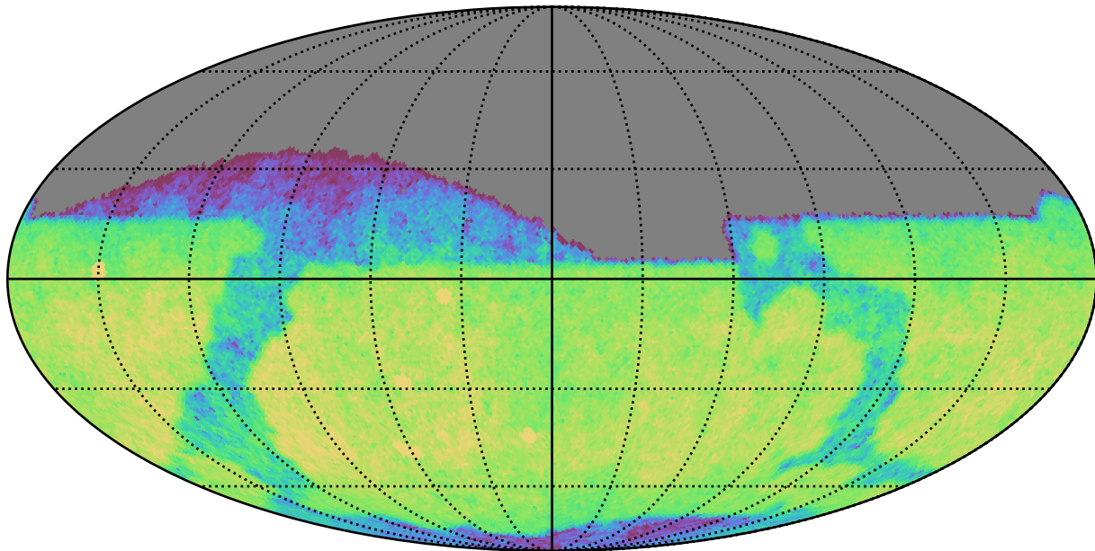
no_magell_roll_v3.4_10yrs Yr 1 i band: CoaddM5
