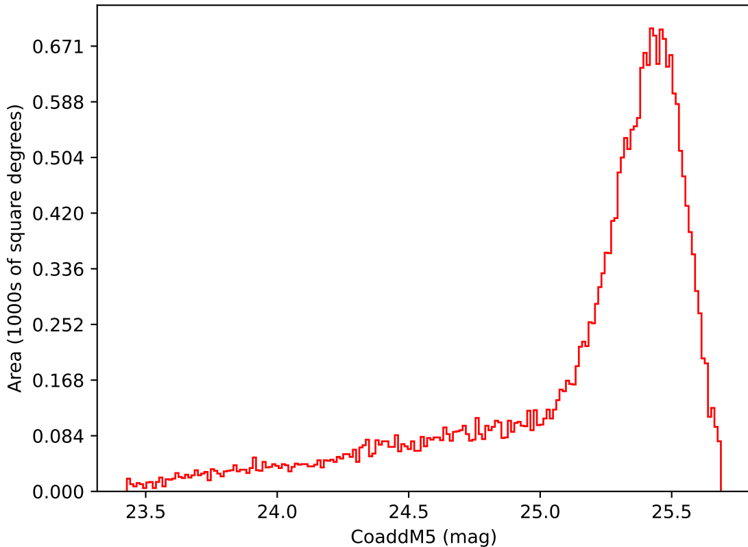
no_magell_roll_v3.4_10yrs Yr 1 i band: CoaddM5
