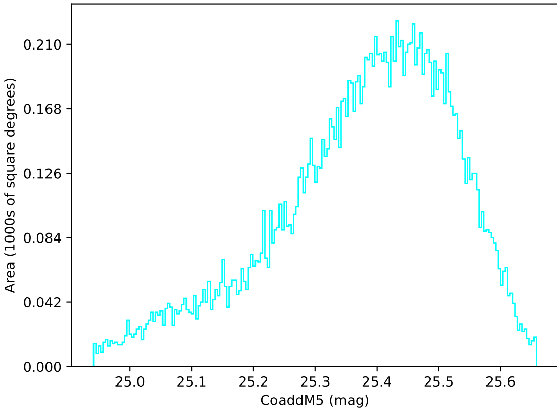
no_magell_roll_v3.4_10yrs WFD u band: CoaddM5
