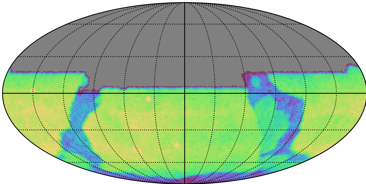
no_magell_roll_v3.4_10yrs All sky u band: CoaddM5
