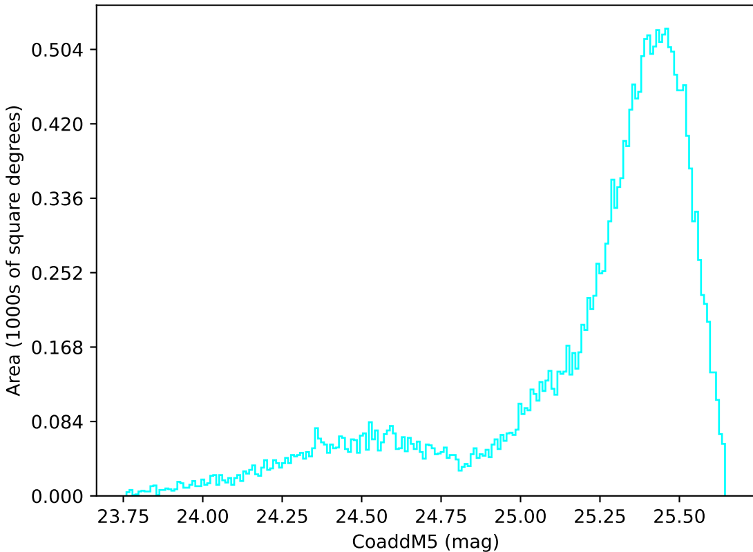
no_magell_roll_v3.4_10yrs All sky u band: CoaddM5
