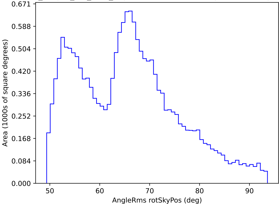
no_magell_roll_v3.4_10yrs WFD all bands: AngleRms rotSkyPos
